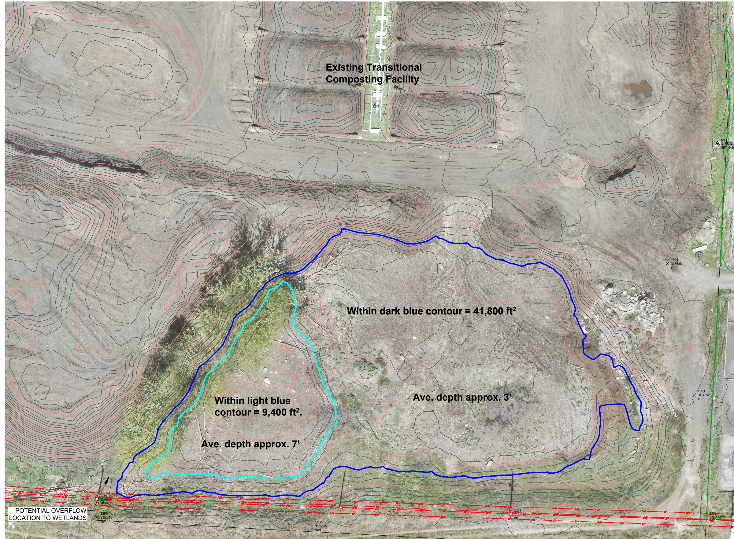
Site Plan - Old Sludge Storage Pond
